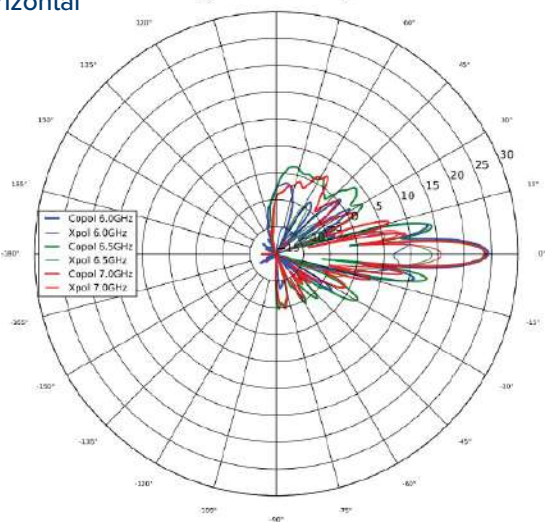
Elevation Horizontal
