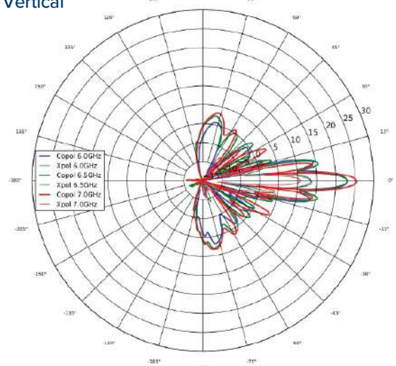
Azimuth Vertical
