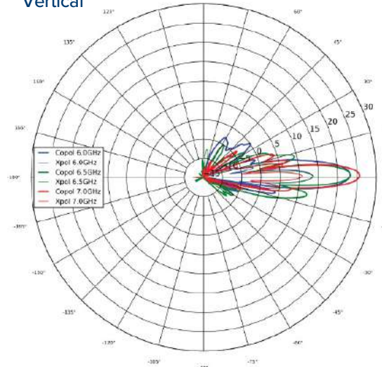
Elevation Vertical
